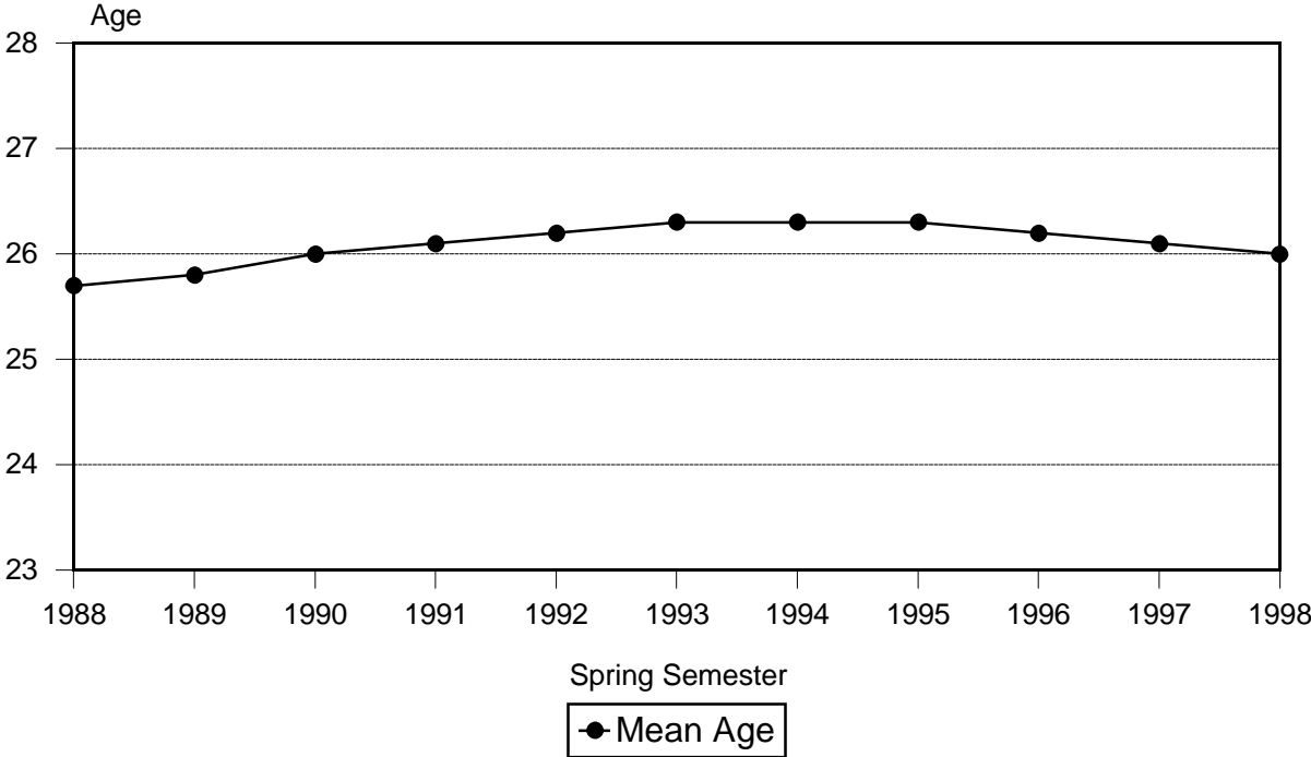
Figure 7 Mean Age
