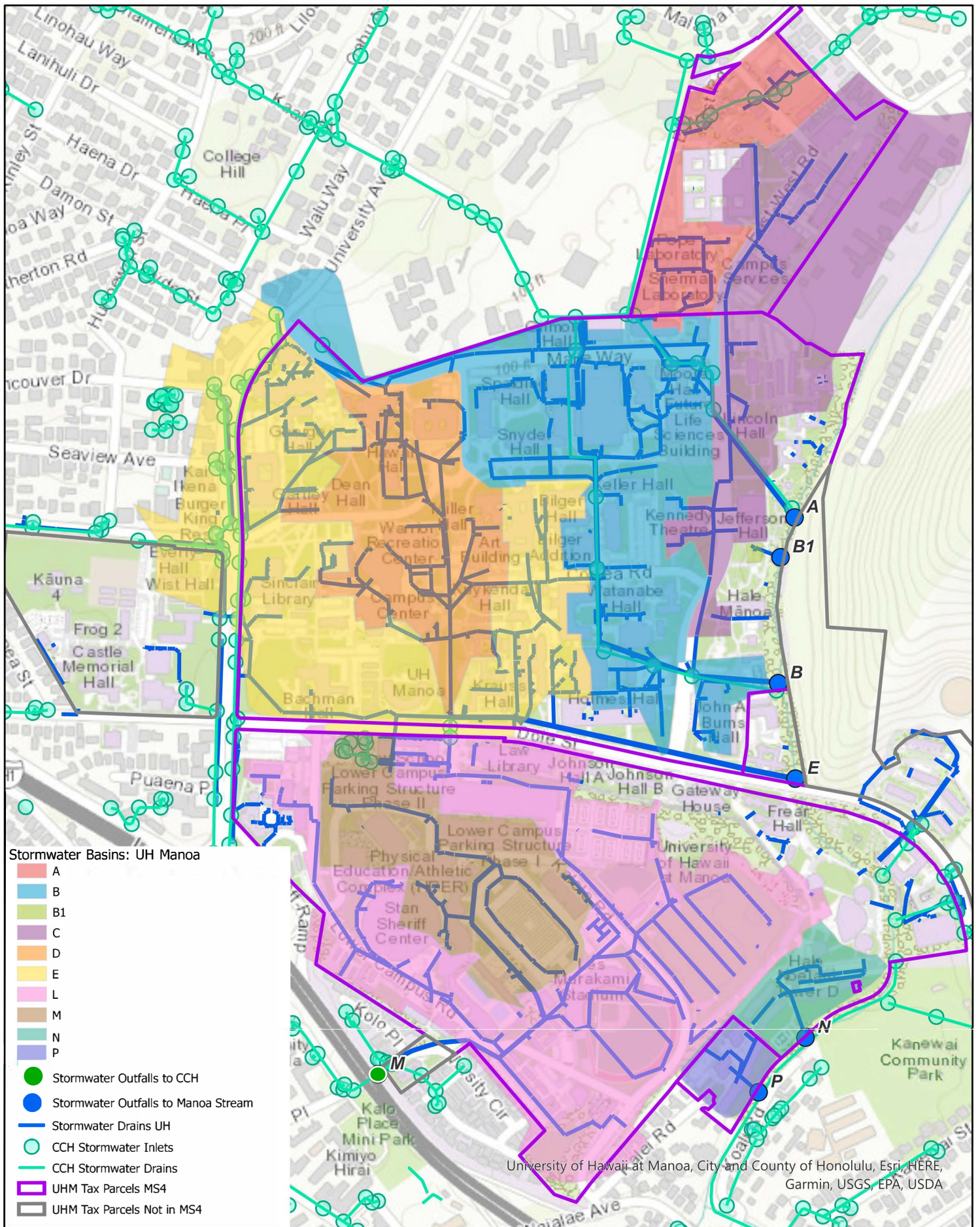
Figure 2 University of Hawaii - Manoa Stormwater Network
