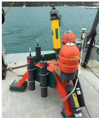
Figure 6. Acoustic device deployed at wave energy test site.
