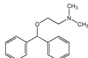
(F) Diphenhydramine
