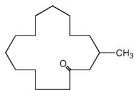
(A) Muscone
