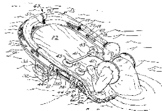
United States Patent 3,155,992 (1962) Life Raft, filed by Glenn A. Shewmake and Matthew I. Radnofsky
