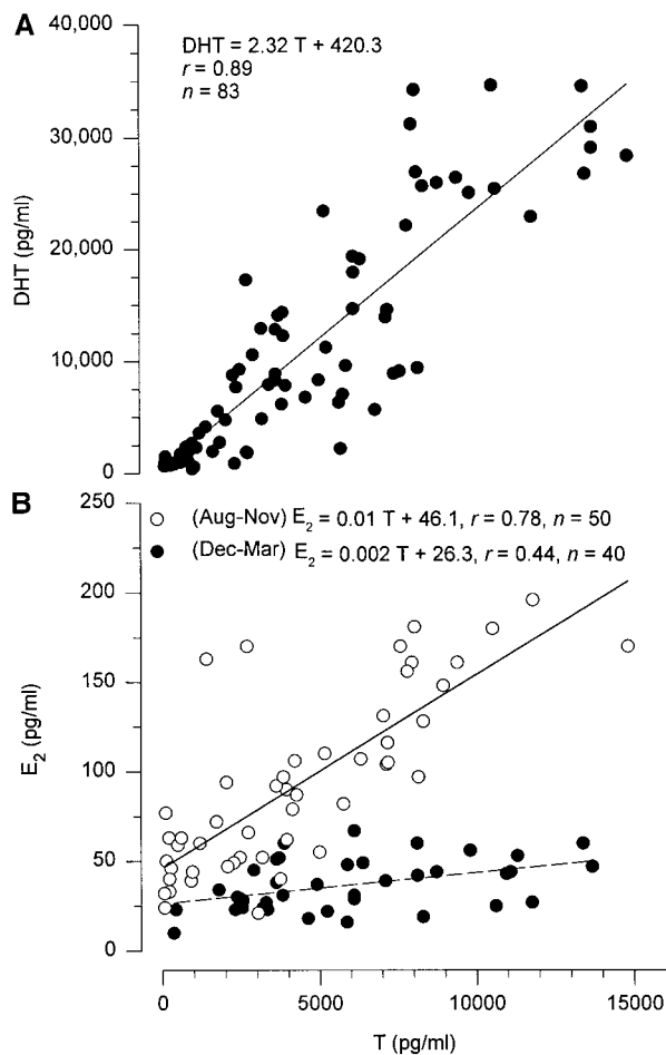
FIG. 2. The association between serum concentrations of androgens and estradiol for male Atlantic stingrays, Dasyatis sabina , collected from the Banana River estuary from August 1993 to March 1994. (A) Relationship between dihydrotestosterone (DHT) and testosterone (T) shows that these androgens covary in concentration throughout the year. Note that DHT concentration is on average approximately 2.3 times greater than T. (B) Relationship between estradiol ( E_2 ) and T shows that productions covary at different rates across the year. Note that E_2 production is approximately 5 times greater during the early phase of gonad development (August–November) compared to the remainder of the reproductive season (December–March). Linear regressions, correlation coefficients, and sample sizes ( n ) are shown.
