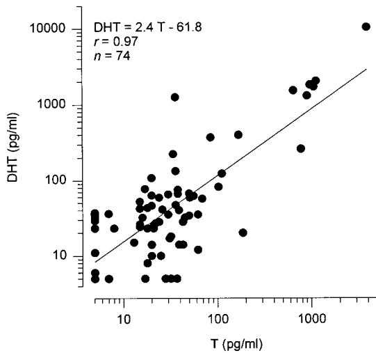
FIG. 5. The association between serum concentrations of testosterone (T) and dihydrotestosterone (DHT) for female Atlantic stingrays, Dasyatis sabina , collected from the Banana River estuary. Concentrations of these two androgen steroids covary across the year. Linear regression, correlation coefficient, and sample size ( n ) are shown.
