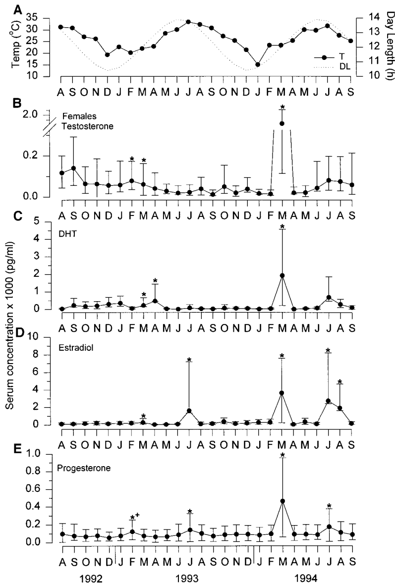
FIG. 4. Serum steroid hormone concentrations (median, 25th, and 75th percentiles) in female Atlantic stingrays, Dasyatis sabina , collected from the Banana River estuary between August 1992 and September 1994. (A) Monthly water temperature and day length profiles across the sampling period as shown in Fig. 1A. (B) Female testosterone and (C) dihydrotestosterone (DHT) levels show a periodic cycling that peaks in February, March, or April. Note the close covariation in androgen levels, especially during 1994. (D) Estradiol levels show two annual surges during March and July of each year and occur during ovulation and parturition, respectively. (E) Progesterone shows coincident peaks with E_2 in February–March and July of each year. All four steroids in females show an annual surge in February–March, whereas E_2 and P_4 show a second annual surge in July. * P < 0.05 as determined by nonparametric analysis in A, B, and C of the entire 26-month data set and Dunn's multiple comparison test. ** P < 0.05 as determined by parametric ANOVA and SNK paired comparisons test in D for the months of December 1992–April 1993.
