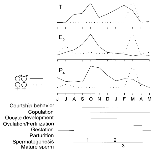
FIG. 6. Summary diagram of the 1993 sex steroid cycles and the associated reproductive events for the study population of Atlantic stingrays, Dasyatis sabina . As male testosterone (T) increases in August, males initiate the mating season 1 month later with biting and courting of females in September. Copulation begins in October when male T, estradiol ( E_2 ), and progesterone ( P_4 ) peak and continues throughout the period of elevated T until the end of April. Periods of maximum gonad size (1), maximum mature sperm presence in testes (2), and maximum seminal vesicle diameter (3) are indicated, as reported by Maruska et al. (1996). Spikes in female T, E_2 , and P_4 are associated with ovulation in March, whereas E_2 and P_4 are also associated with parturition in July.
