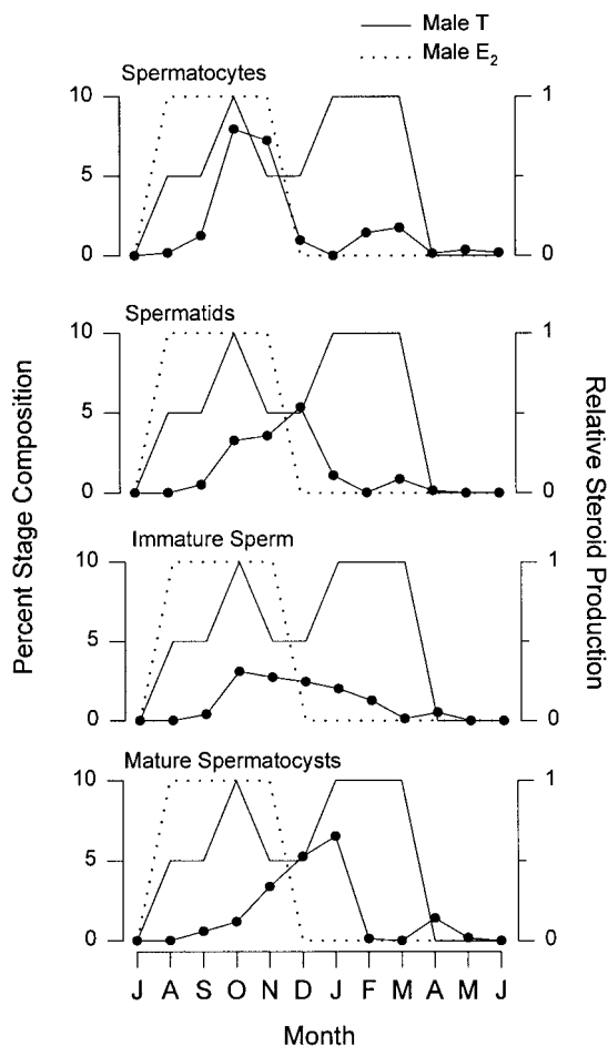
FIG. 3. Stages of testes development and changes in steroid levels in male Atlantic stingrays, Dasyatis sabina , collected from the Banana River estuary from July 1993 to June 1994. Four histological stages of spermatogenesis (SIII–SVI of Maruska et al. , 1996) are expressed as percentage of total gonad weight for each monthly sample (closed circles). Steroid concentrations for T and E 2 are expressed as differences among months as determined by statistical analyses for this period in Fig. 1 and are expressed in relative values. Note that the October peak in T is coincident with peak activity of primary and secondary spermatocytes, whereas the second January–March peak in T is coincident with a relatively brief activity of spermatocytes and peak of sperm maturation. E 2 production is associated only with the first production of spermatocytes.
