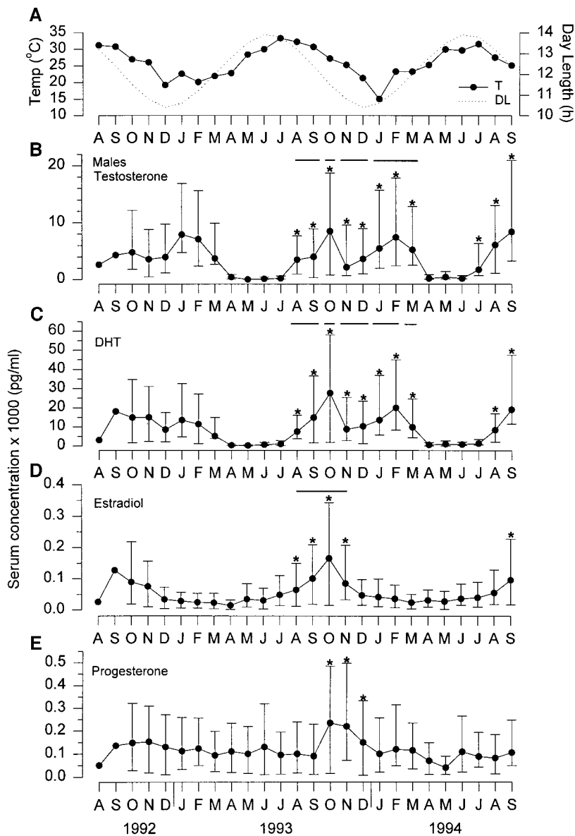
FIG. 1. Serum steroid hormone concentrations (median, 25th, and 75th percentiles) in male Atlantic stingrays, Dasyatis sabina , collected from the Banana River estuary between August 1992 and September 1994. (A) The monthly water temperature (T) and day length (DL) profiles across the sampling period. Maximum day length (13.5 h) and annual temperatures ( >30^{\circ}\text{C} ) occurred during the months of June and July, respectively. Shortest day length (10.5 h) occurs in December and lowest water temperatures were recorded during December 1992 and February 1994. (B) Testosterone (T) and (C) dihydrotestosterone (DHT) levels in the sample population show a periodic cycling that begins in August and has a major peak in October and a second minor peak in January–March. Note the close covariation in changes in T and DHT. Bars above T and DHT levels show which months differ and support the existence of bimodal peaks during the period of androgen surge. (D) Estradiol shows a broad, monophasic cycle that peaks in October. (E) Progesterone is detectable in the serum throughout the year and peaks in October 1993 along with the other steroids. * P < 0.05 .
