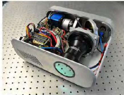
Field Test Unit
