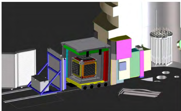
Simulated tests at a nuclear reactor
